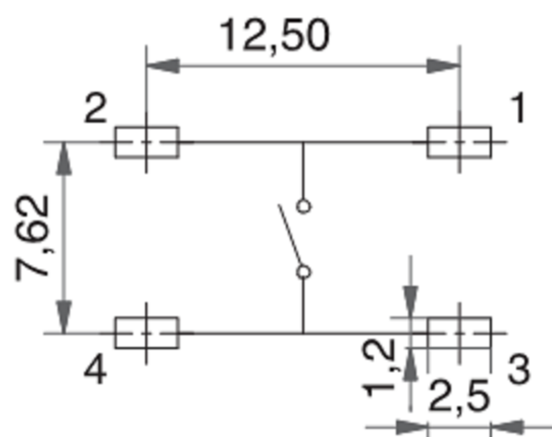
SMD PCB
